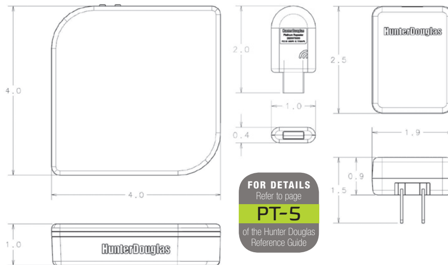
Platinum App components: the Platinum App Bridge, Platinum Repeater and its power source.
